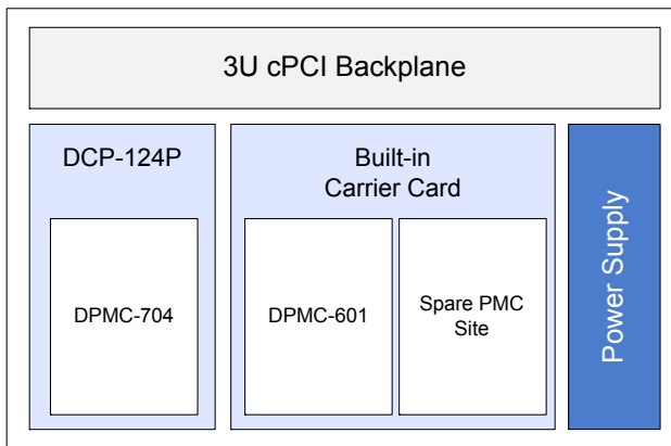
Figure 1: MPMC-9310-0010 Block Diagram
